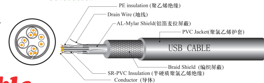
CK15-050 USB AM/BM
